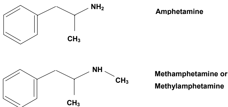
Figure 1. Amphetamine and methamphetamine molecules
