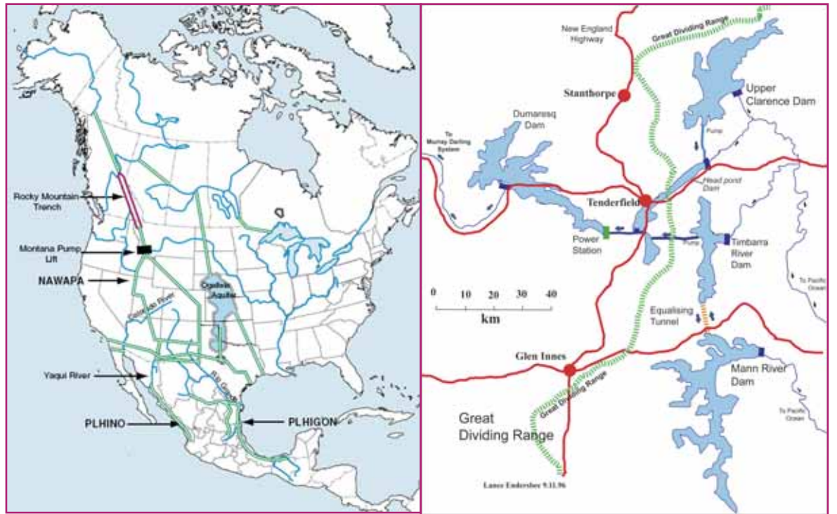
Schematics for the NAWAPA (left) and Australia's Clarence River Scheme (right). The sheer scale of NAWAPA will transform the entire Biosphere; Australia can participate in this Biospheric development through projects such as the Clarence scheme.
