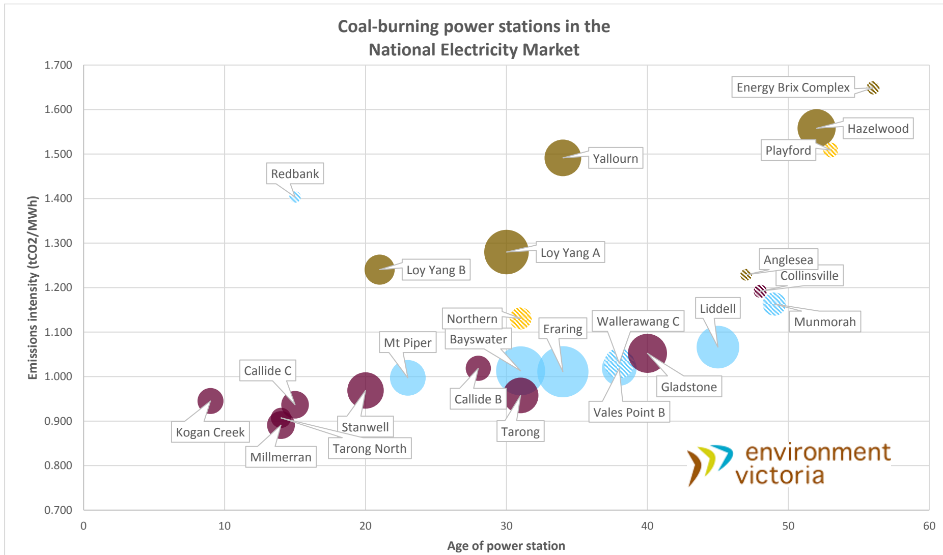
Figure 1. Coal-burning power stations in the NEM. The size of each circle represents the capacity of each generator. Victorian generators = brown circles; NSW = blue circles; QLD = maroon circles; SA = gold circles. Power stations that have closed in the past two years are represented by the diagonal lines through the circles.
