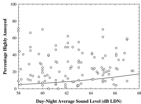
Figure 4: Percentage highly annoyed at aircraft noise plotted as a function of noise level. The solid curve is a portion of that presented in Figure 3, while the scattered points represent real measurements (data from Fidell, 2003).
