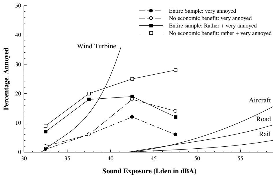
Figure 2: Annoyance plotted as a function of noise level for four theoretical models (rail, road, air: Miedema and Oudshoorn, 2001; wind turbines: Pedersen et al., 2004) and four sets of data obtained from van der Berg et al., (2008). For the data, closed symbols are for the entire sample, while open symbols are for those who identified that they had no economic interest. Circles represent the percentage of “very annoyed” responses whilst squares represent the sum of “very annoyed” and “rather annoyed” responses.
