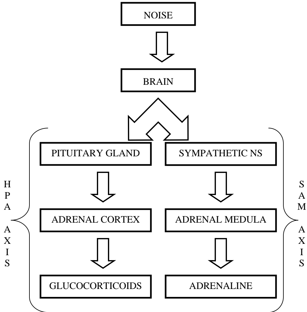
Figure 10: Schematic representation of the body’s response to unwanted sound. Both the HPA axis and the SAM axis are regulated by a brain structure known as the hypothalamus.
