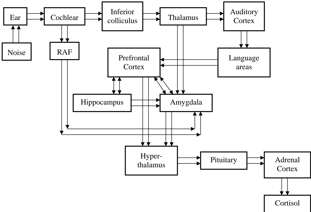
Figure 11: The link between noise and the hypothalamic-Pituitary-Adrenal (HPA) axis. Note: RAF = reticular activating formation.
