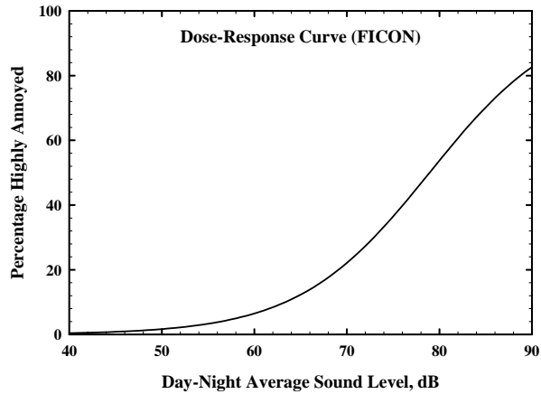
Figure 3: A theoretical curve formulated to model the relationship between noise level and annoyance to aviation noise.
