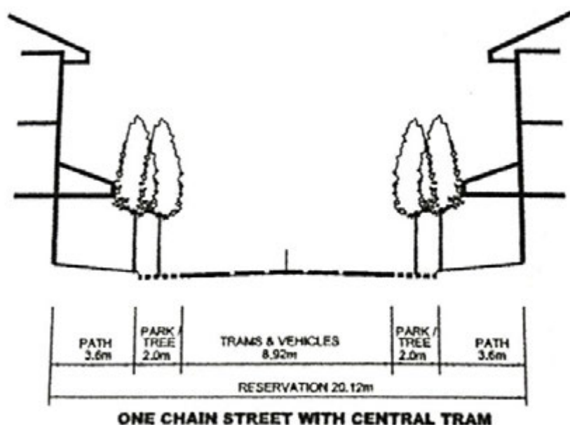
Figure 22: One Chain (20 metre) street with central tram
