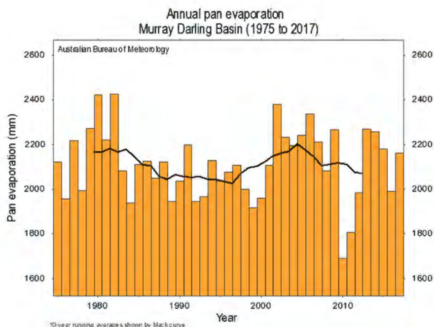
Figure A5.11 Annual pan evaporation, Murray-Darling Basin (1975-2017) Source:
