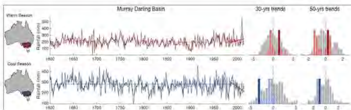
Figure A5.4 Regional rainfall reconstructions (Freund et al. 2017)
