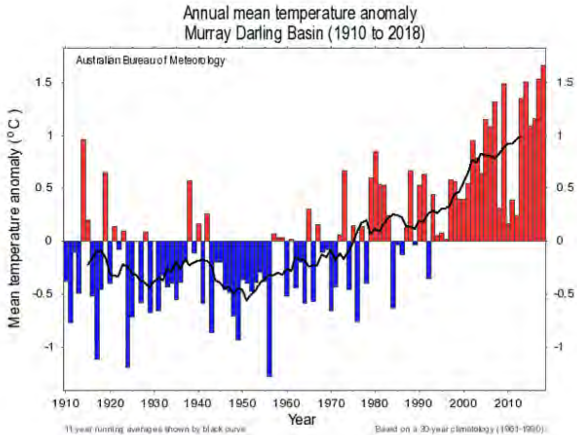
Figure A5.6 Annual mean temperature anomaly, Murray Darling Basin (1910-2018).
