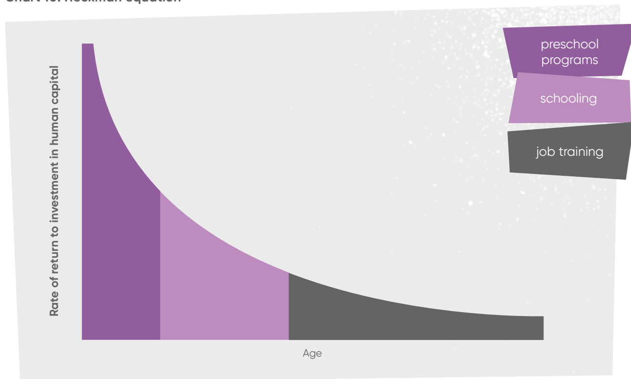
Chart 10: Heckman equation
