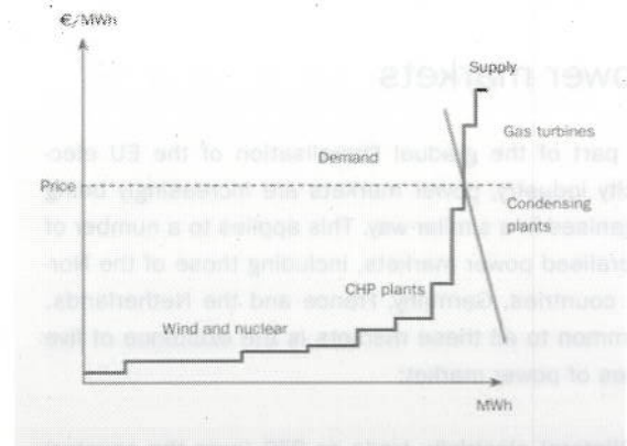
FIGURE 3: ANNUAL SUPPLY AND DEMAND CURVES IN THE POWER MARKET
