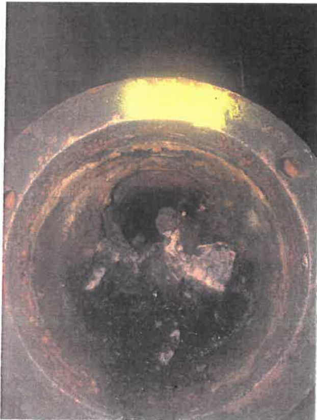
Footage of existing conditions of trade waste line from MGK
