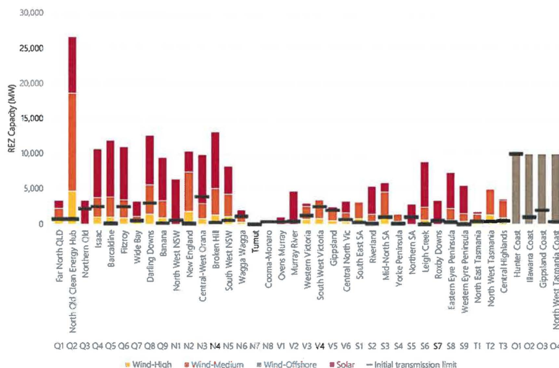
Figure 6: National Electricity Market (NEM) Renewable Energy Zone potential resource quantity and transmission limits, showing that the Hunter offshore area with the highest available initial transmission limit in the NEM.
