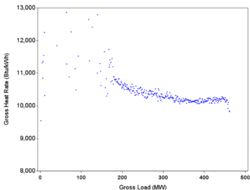
Figure 2-3. Gross Heat Rate vs. Load (MW): EW Brown Unit 3 (Bituminous, Subcritical Tangential-fired)
