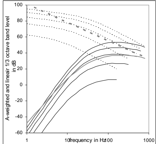
Figure VIII.2: calculated linear (dashed) and A-weighted (solid lines) 1/3-octave pressure levels due to atmospheric turbulence on a screened microphone with F(z)+C=42 \text{ dB} , D = 0.1 \text{ m} and wind speeds 2, 4, 6, 8, 10 m/s (black, bottom to top); bold grey lines: 1/3 octave band levels according to Strasberg for 10 m/s
