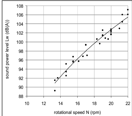
Figure IV.3: measured wind turbine sound power level L_W as a function of turbine rotational speed N
