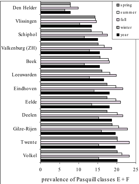
Figure VI.10: prevalence of observed stability (Pasquill classes E and F) per season and per year at 12 different Dutch stations over 30 years (data from [KNMI
