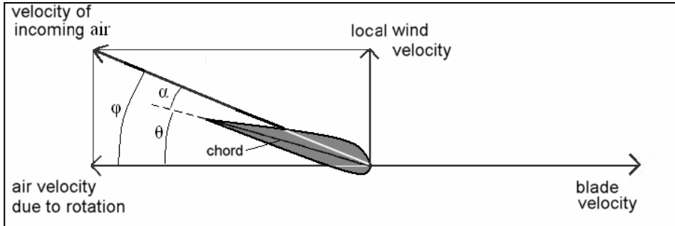
Figure III.2: flow impinging on a turbine blade with flow angle \varphi , blade pitch angle \theta and angle of attack on blade \alpha = \varphi - \theta
