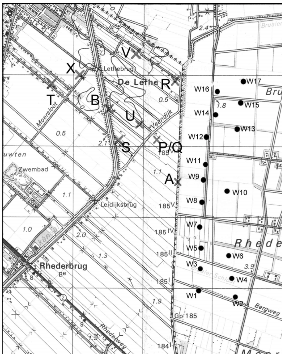
Figure IV.2: turbines (dots W1....W17) in and measurement locations (crosses A....X) near the Rhede wind farm; Duch – German border indicated by line of +++ (through A); grid lines are 1 km apart, north is at top
