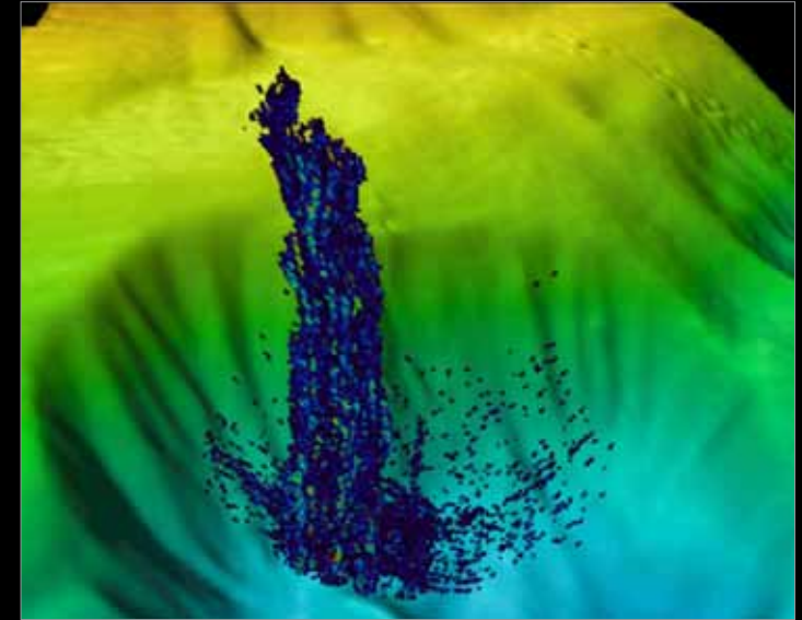
Methane hydrate collapse, off California, 2009. (NOAA)
